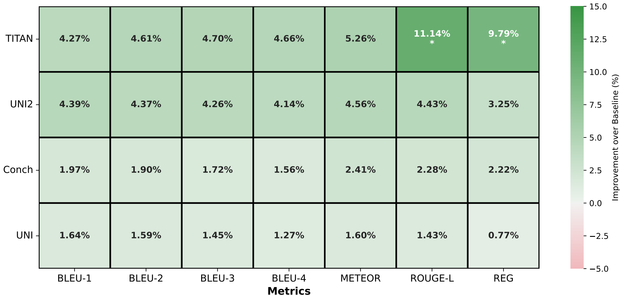
Percentage Improvement Over HistGen Baseline (with Statistical Significance)
